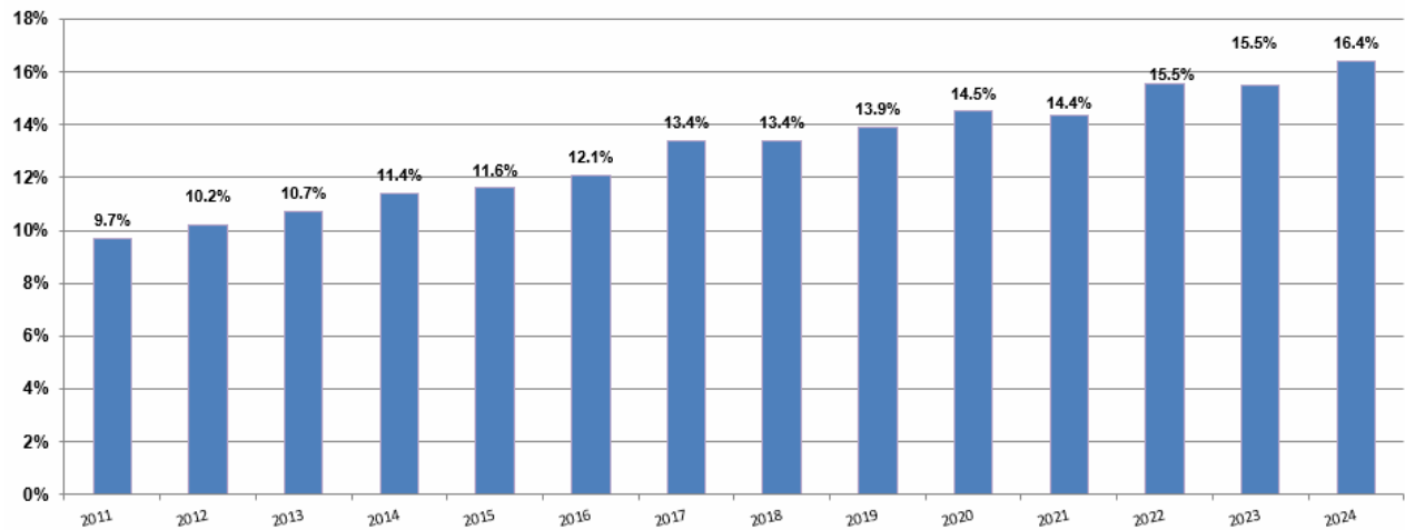
Figure1. Statewide Biofuel Distribution Percentage, 2011-2024 Calendar Years
